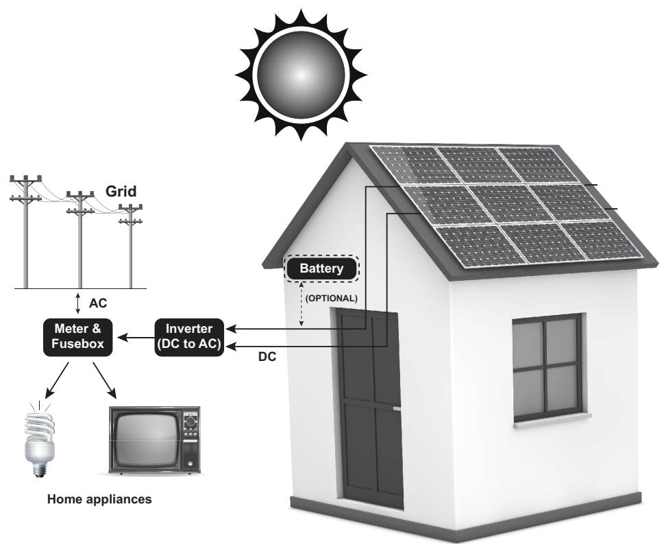
TYPICAL GRID CONNECTING PHOTOVOLTAICS SOLAR SYSTEM
